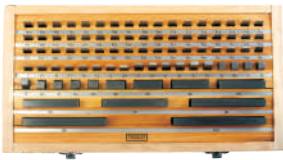
Steel Slip Gauge Box
